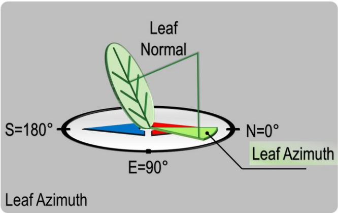
Fig. 25: Leaf Azimuth
