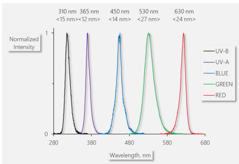
Fig. 20: Emission spectra of LEDs involved in screening measurements
