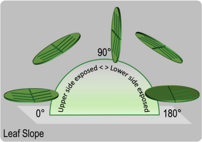
Fig. 24: Leaf Slope
